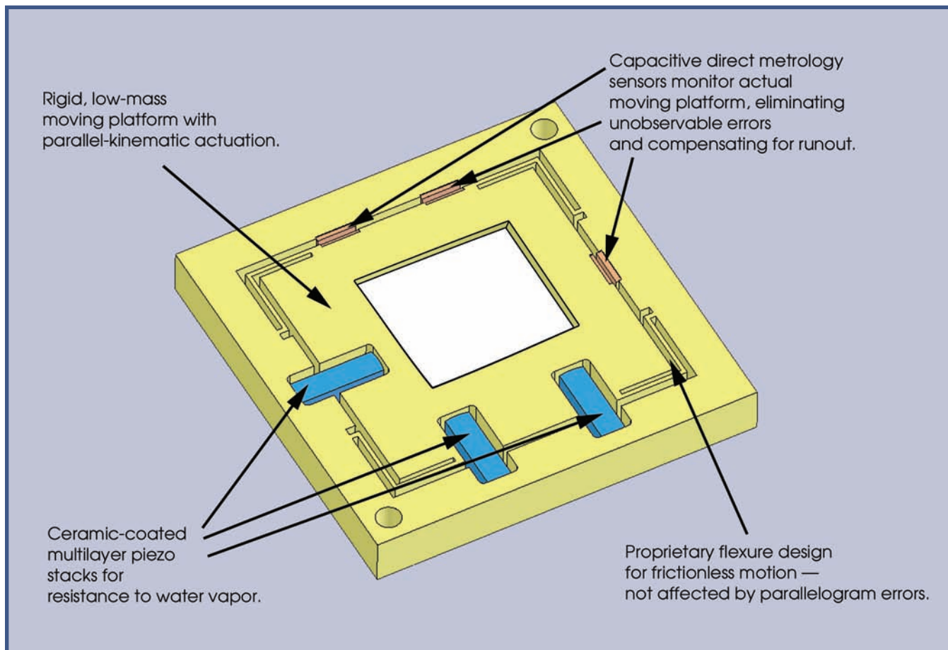
Figure 1. Nanopositioning stages with capacitive sensors for high resolution, bandwidth and stability enable optical trapping applications. Parallel-kinematics/parallel-metrology designs offer superior motion fidelity by positioning and measuring a single platform — using multiple actuators and sensors — against the same stationary reference.
